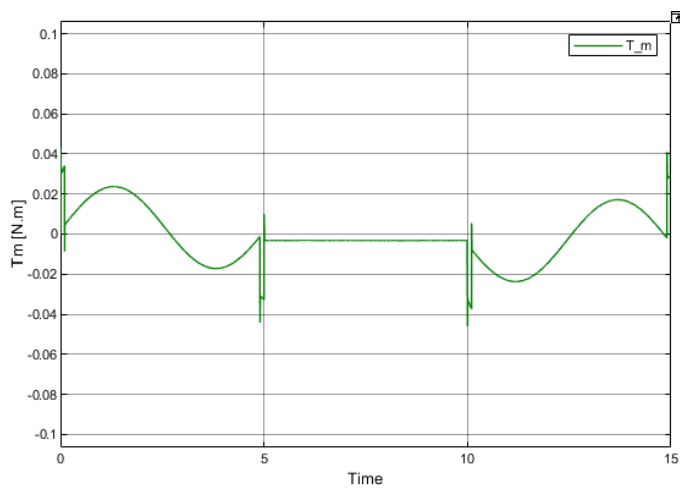
Figura 55: Torque motor T_m
